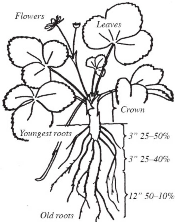
Figure 8.1. The strawberry plant and its root distribution. (Courtesy of the University of Wisconsin.)
